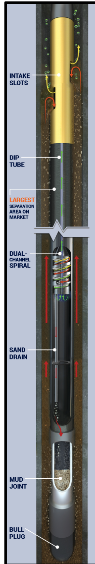
Figure 5: Schematic of the separator
