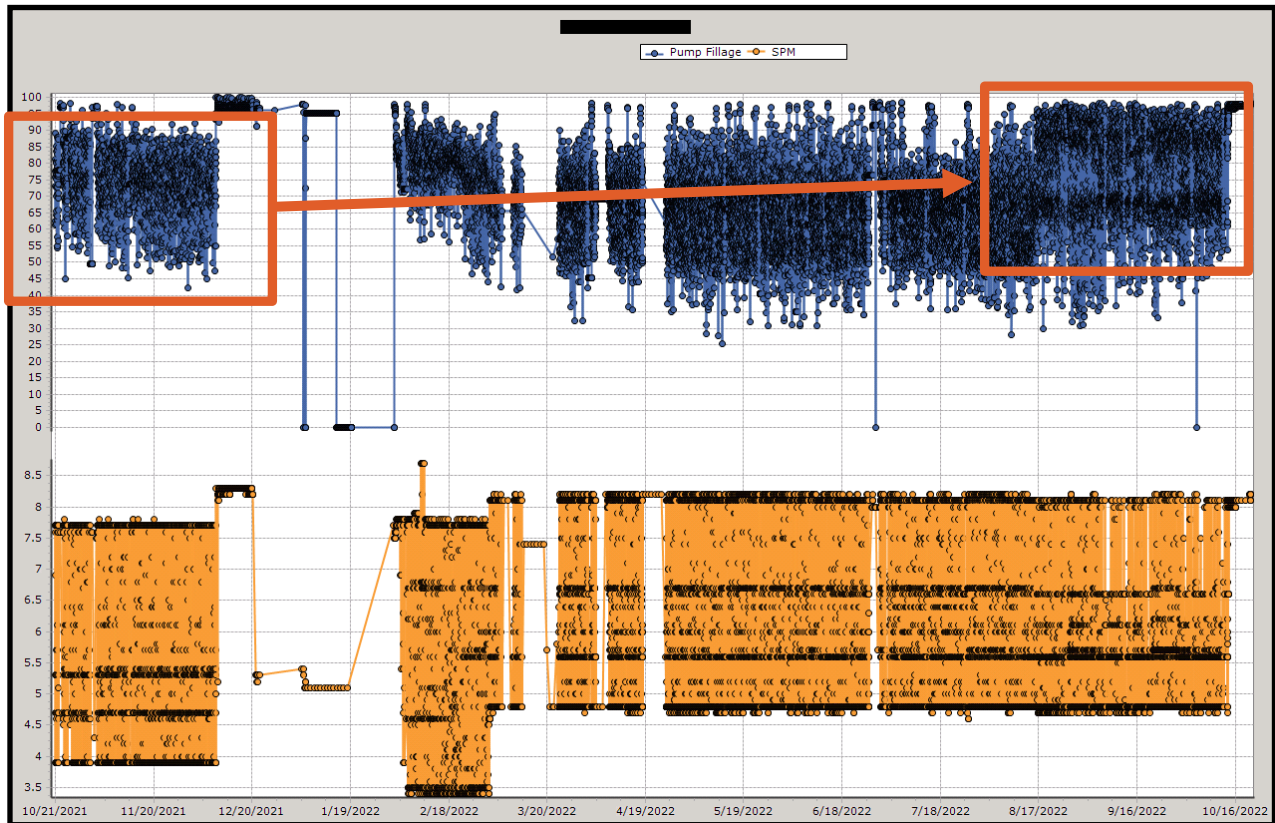
Figure 9 – Pump Fillage and SPM trend for Well 1.
