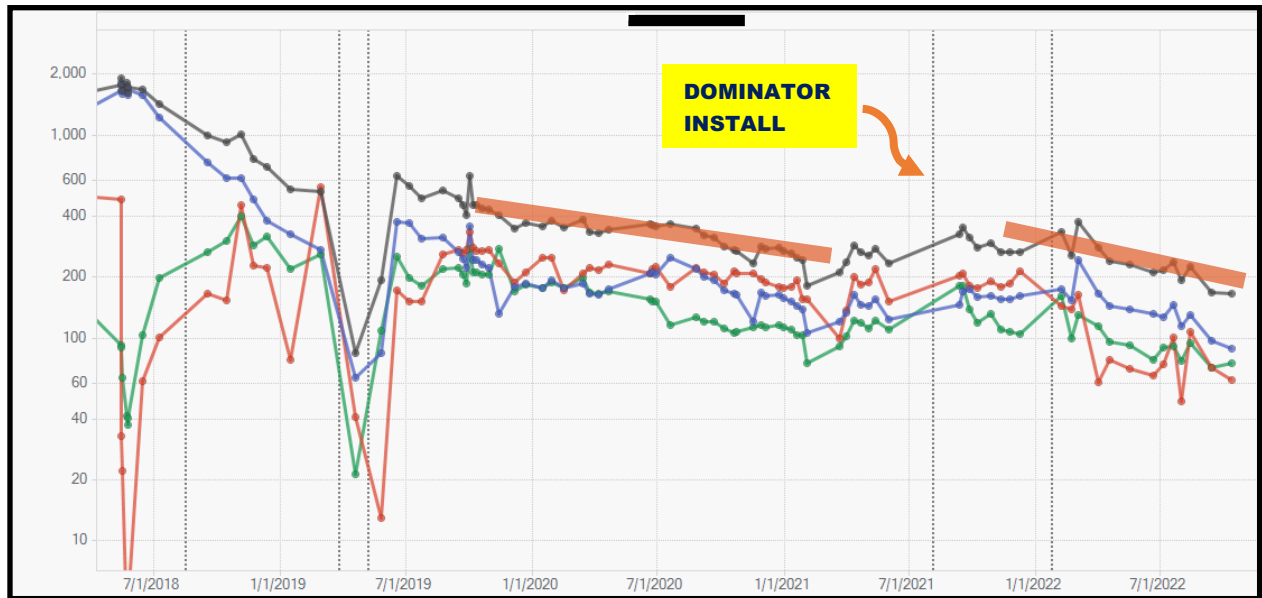
Figure 7 – Production Data from Well 1.
