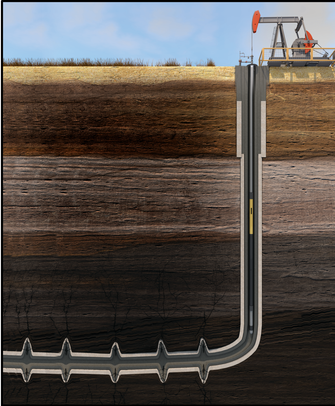
Figure 3: Wellbore showing multiple frac zones and placement of the tool.
