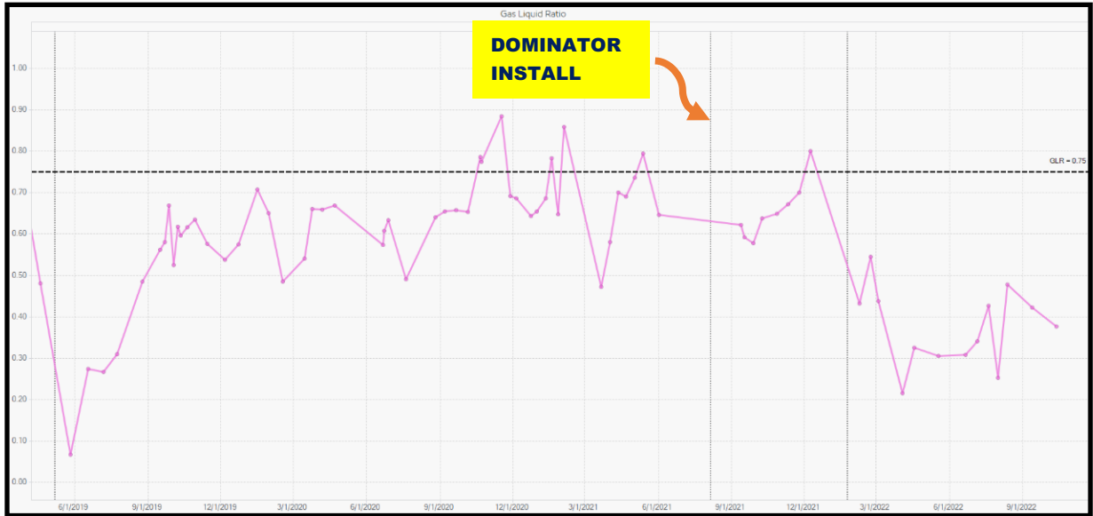
Figure 8 – Gas to Liquid Ratio for Well 1.
