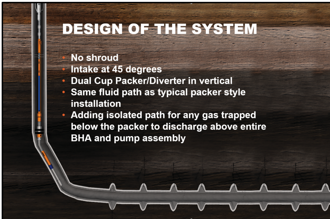
Figure 3: Silver Bullet Tool Diagram
