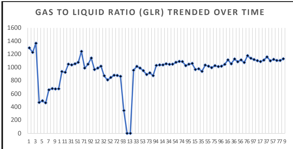
Figure 7: Case Study Gas to Liquid Ratio GLR Curve Over Time
